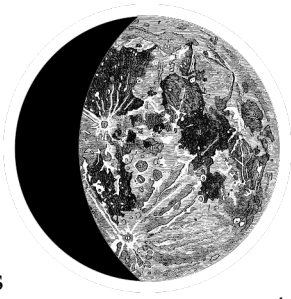
Waxing Gibbous
