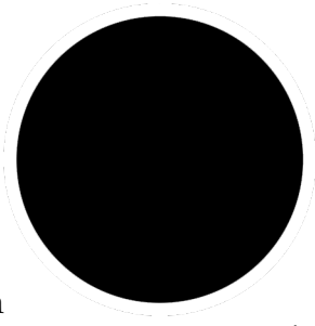
New Moon
