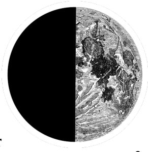
First Quarter
