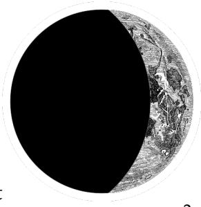
Waxing Crescent
